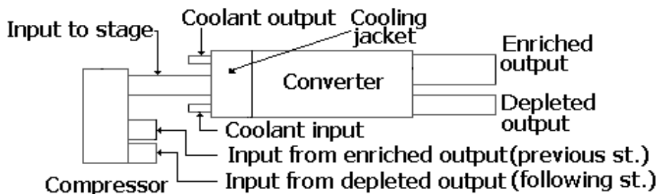
Figure F-3. Schematic layout of a cascade converter or cell with associated compressor. The control valves are not shown.
